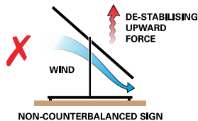
NON-COUNTERBALANCED SIGN
